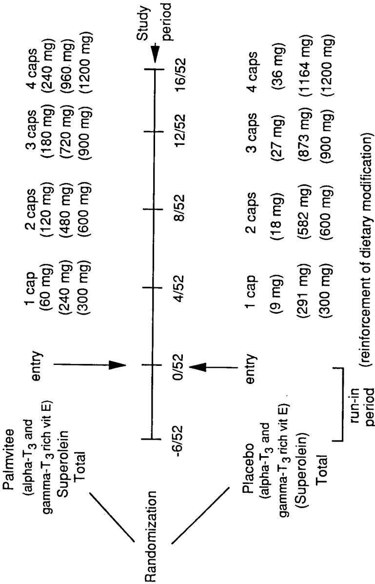
Figure 1: STUDY DESIGN
