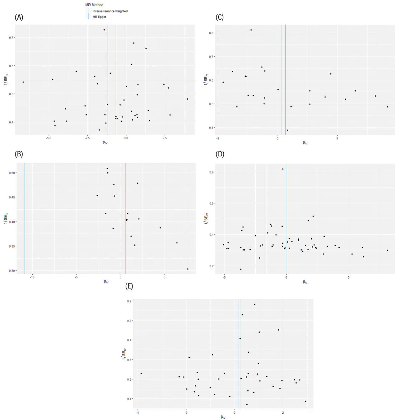
Figure 2. Funnel plots of two-sample Mendelian randomization results. (A) Funnel plot of dried fruit intake and ulcerative colitis. (B) Funnel plot of vegetable intake and ulcerative colitis. (C) Funnel plot of processed meat intake and ulcerative colitis. (D) Funnel plot of fresh fruit intake and ulcerative colitis. (E) Funnel plot of cereal intake and ulcerative colitis
