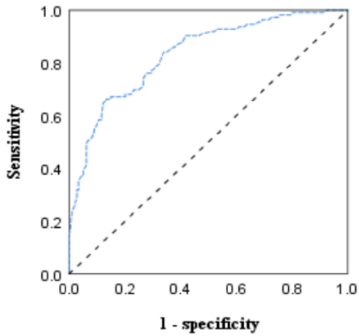
Figure 1. ROC curve of serum 25(OH)D in predicting prediabetic CAN.
