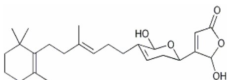
Fig.8. Manoalide
